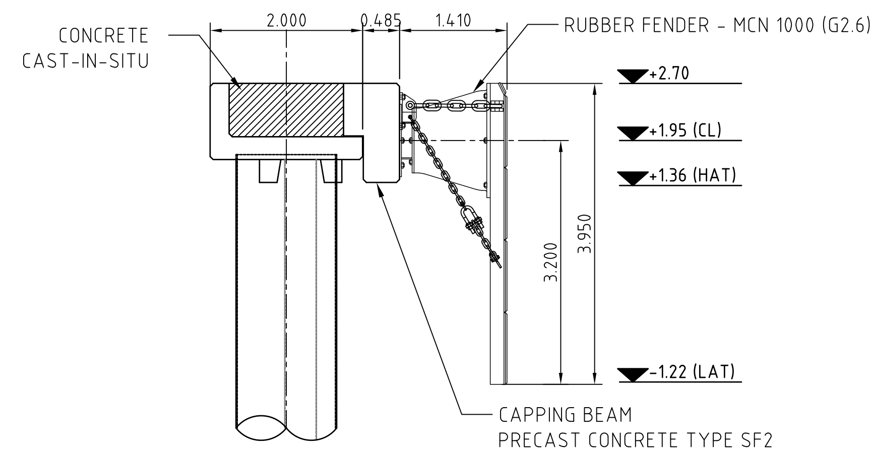
SECTION (A) 1:50 -
